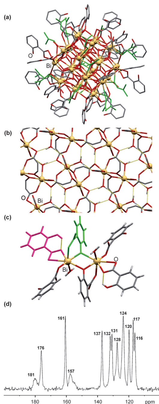
Figure 3. a) A single \text{Bi}_{38}\text{O}_{44}(\text{Hsal})_{26}(\text{H}_2\text{O})_4(\text{DMF})_{18} cluster in 4 , with coordinated DMF shown in green; b) a polymeric sheet of 2 viewed along the crystallographic a axis, displaying only the sections of Hsal − and sal 2− ligands directly involved in coordination and hydrogen (shown in yellow) bonding; c) a fragment of a sheet of 2 highlighting different bonding modes of sal 2− (green) and Hsal − (purple) anions; and d) ^{13}\text{C} CP-MAS SS NMR spectrum of 2 .
